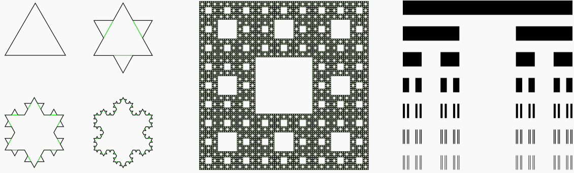
FIGURE 1.10. Fractal shapes: the Koch snowflake (left) of Hausdorff dimension \frac{\log 4}{\log 3} \approx 1.26 , Sierpiński carpet (middle) of dimension \frac{\log 8}{\log 3} \approx 1.89 , and middle-thirds Cantor set (right) of dimension \frac{\log 2}{\log 3} \approx 0.63 .
